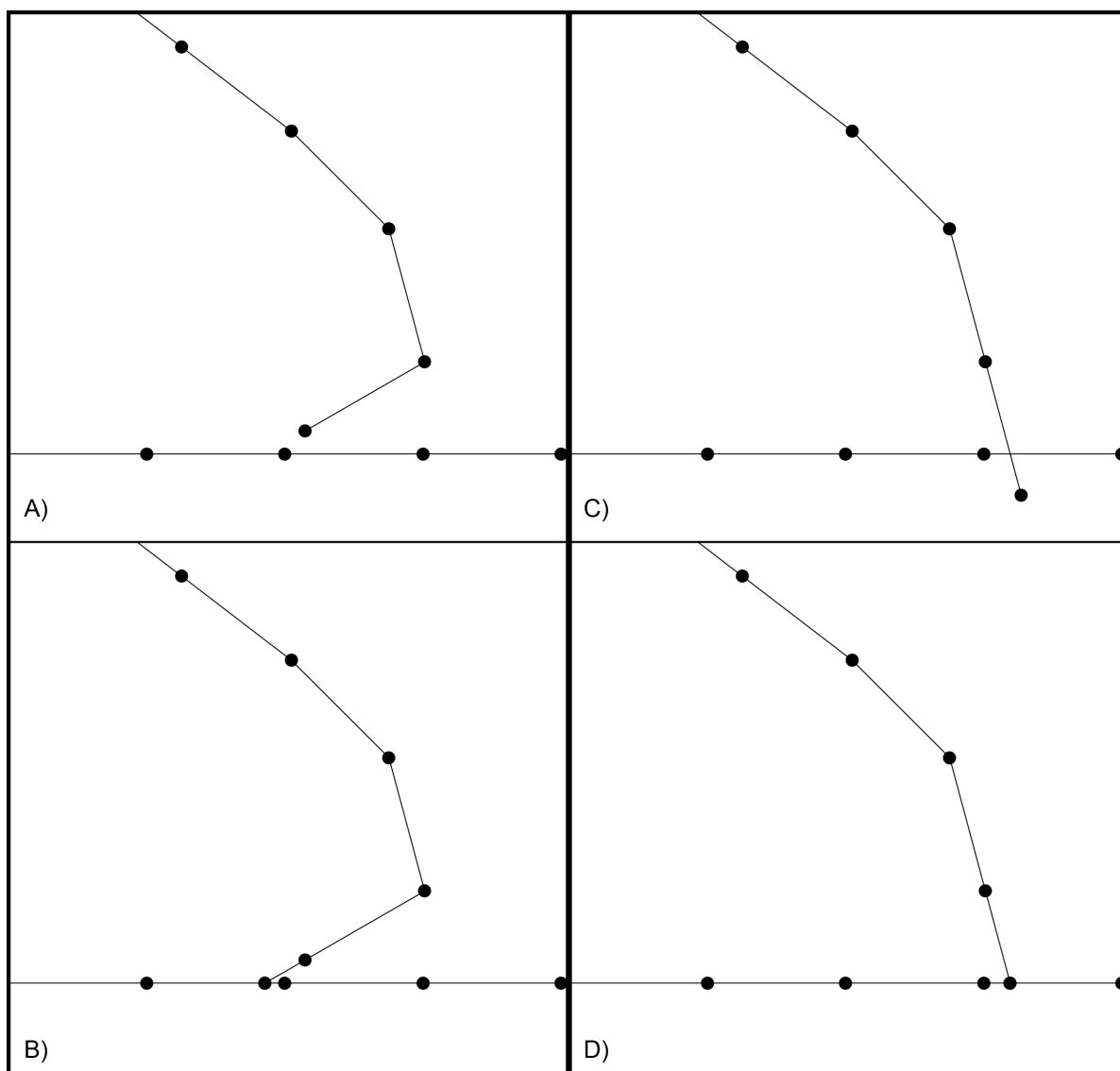
Figure 3: This illustration demonstrates how GROW detects and corrects the intersection of elements of two different faults. A) shows the fault geometry created by adding an element at 255^\circ to the tip of the upper fault. Because the tip of this potential element falls within one element half-length of the lower fault, GROW adds a smaller element to the tip the upper, propagating fault (as shown in B). GROW defines the intersection of the upper and lower fault at exactly one set of coordinates by dividing an element of the lower fault into two smaller elements, but maintaining the location of the previous element nodes of the lower fault. C) shows an example where the potential element intersects pre-existing fault. In this case, as shown in D), the propagating element tip is replaced by a smaller element that exactly intersects the lower fault, and an element of the lower fault is divided into two smaller elements.
